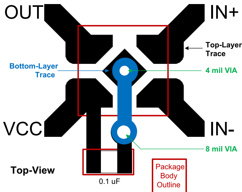
Figure 42. Layout Example
