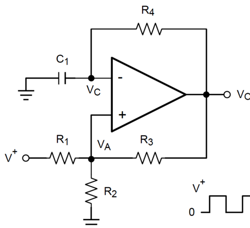
Figure 39. Square-Wave Oscillator
